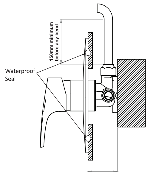
42-69 mm distance from mounting stud to outside face of wall lining
